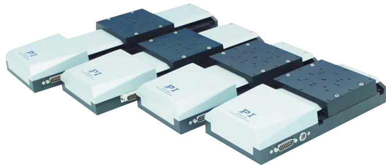
M-505 translation stages with ballscrew drives
