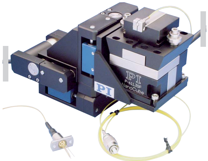
F-130 fiber alignment system consisting of an M-110 XYZ positioning system and a P-611 XYZ Piezo-NanoPositioning system. This combination can be operated by the C-880 controller or NI controllers (request our technote!)
